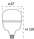
Lampadina a Led 20W, 240V
