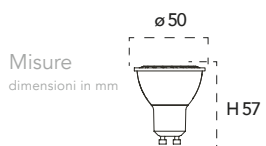
Lampadina a Led 6W, 240V KIT 3
