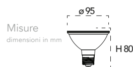
Lampadina a Led 10W, 240V
