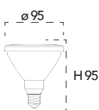
Lampadina a Led 12W, 240V
