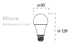
Lampadina a Led 19 W, 240V
