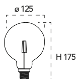
Lampadina a Led 16W, 240V
