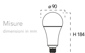
Lampadina a Led 27,5W, 240V
