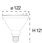
Lampadina a Led 18W, 240V
