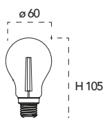
Lampadina a Led 8W, 240V
