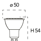
Lampadina a Led 3W, 240V
