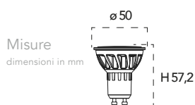
Lampadina a Led 4W, 240V
