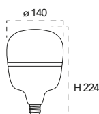
Lampadina a Led 45W, 240V
