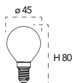
Lampadina a Led 6W, 240V
