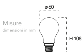
Lampadina a Led 11W, 240V
