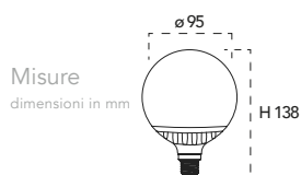
Lampadina a Led 18W, 240V
